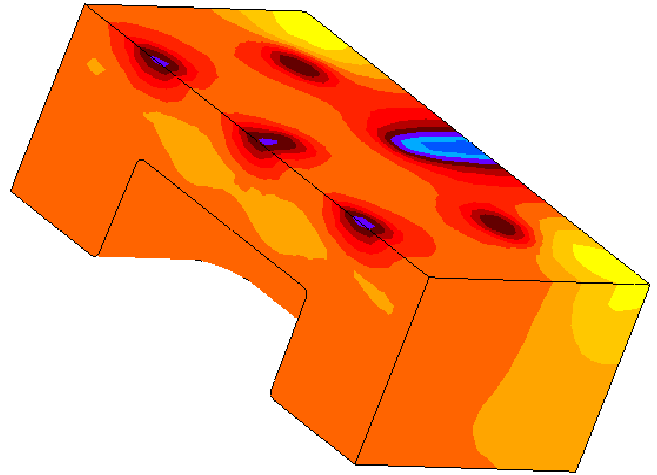
Heating Line Design for a Stamping Die
