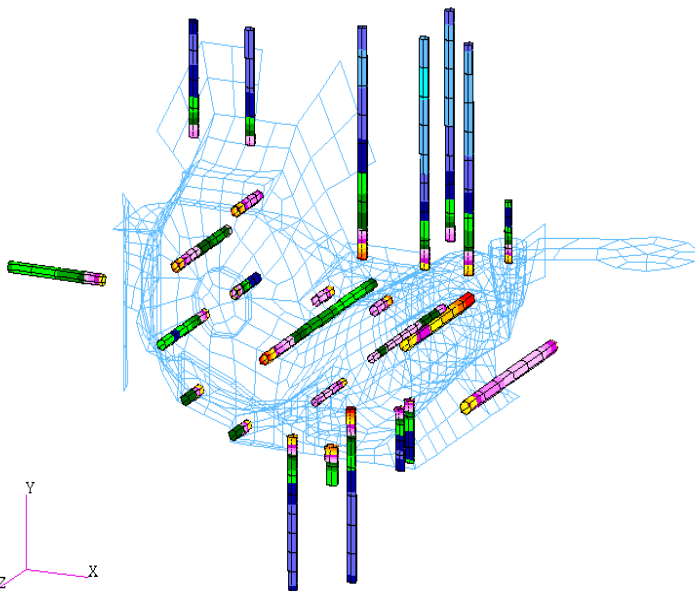
Cooling Line Design for a Die-cast Part
